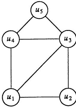
Figure 1. The graph F .
