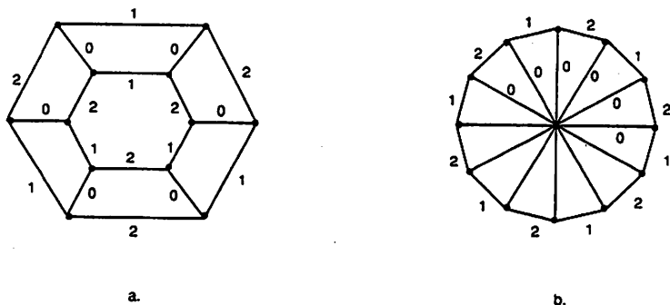
Fig 8. A dual of a map on the sphere.
