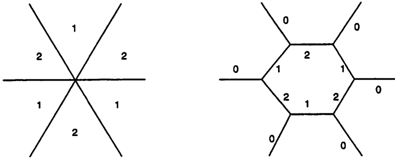
Fig. 4. The 3-graph of a hypermap.
