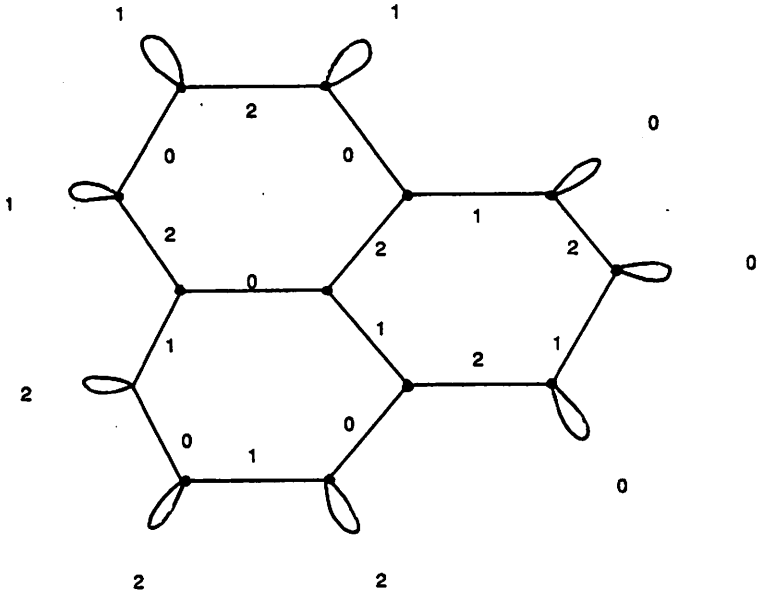
Fig. 2. Non-ordered 3-graph.
