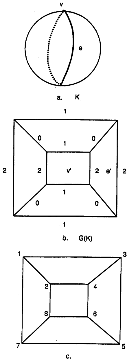
Fig. 1. A map K and the 3-graph that encodes it.
