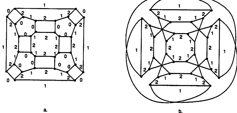
Fig 7. A dual of the pyramid.
