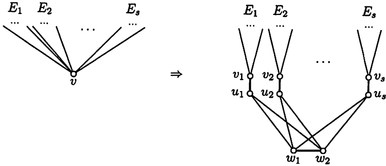
Figure 1: Illustration for the proof of Proposition 3. E_i denotes the set of edges of color i incident with v .
