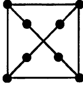
Figure 3: Planar, but not isometrically embeddable in the plane
