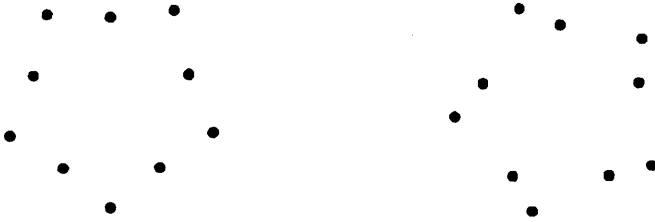
Figure 5: Euclidean vertices with D_5, \mathbb{Z}_5 isometry group respectively
