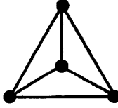
Figure 1: Symmetric, but not isometric, embedding of K_4
