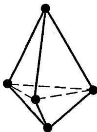
Figure 2: An isometric embedding of K_{2,3}
