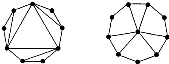
Figure 4: \mathbb{Z}_3 -symmetry and D_3 -symmetry.
