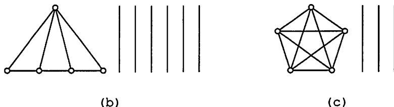
FIGURE 1. Configurations (b) and (c) of Proposition 4.1.
