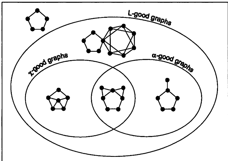
Figure 1: Intersection between classes of good graphs.
