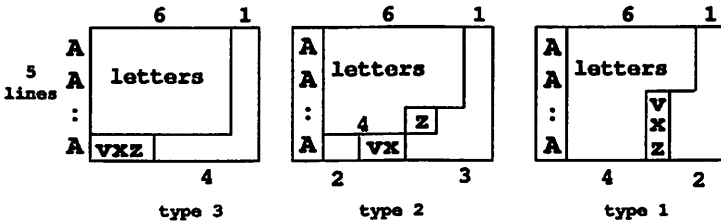
Figure 14: A-line solution patterns for PP(7)
