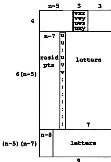
Figure 6: An arrangement of the residual lines in PP(n) , where n \geq 7 .
