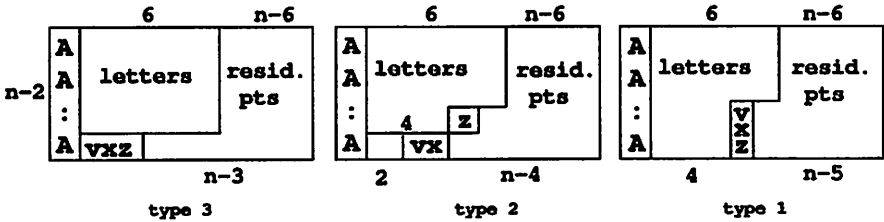
Figure 8: The possible A-line solution patterns
