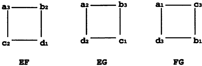
Figure 21: PP(7) , pairs of a_i, b_i, c_i, d_i in the E, F, G -lines
