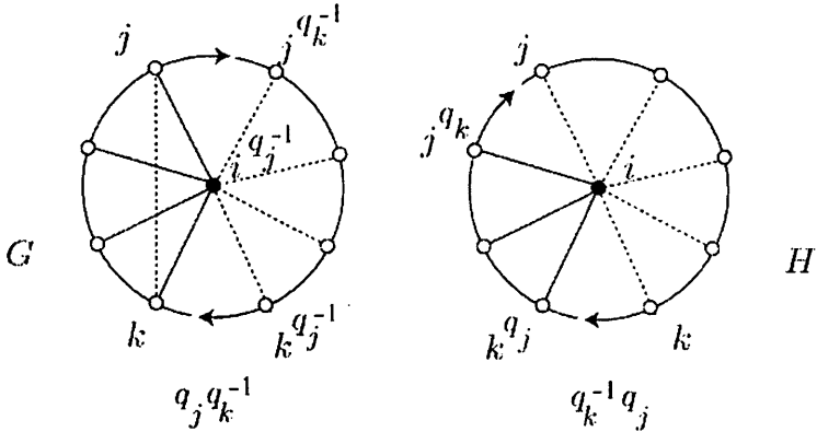
Figure 13, i^{q_j^{-1}} = i^{q_k^{-1}}
