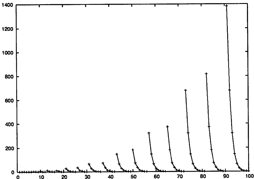
Figure 2. e(n) for n \leq 100 .
