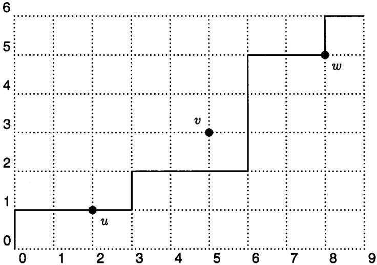
Figure 3: The Three-Points Lemma for \tau = 3 and s = 2
