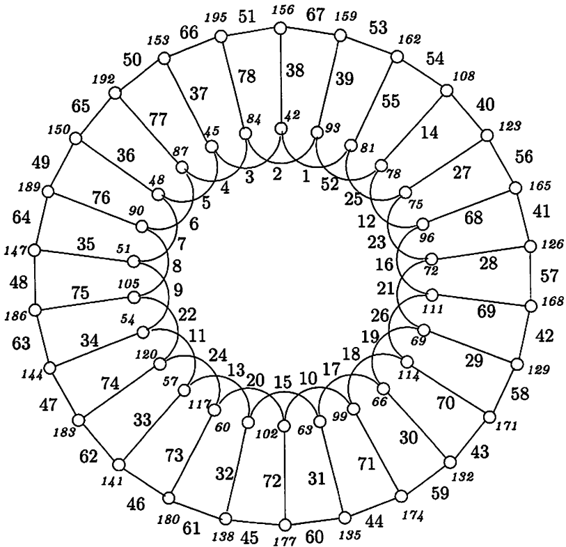
Figure 2.3 : The (\frac{3n+6}{2}, 3) -antimagic labeling of the graph P(26, 2) .
