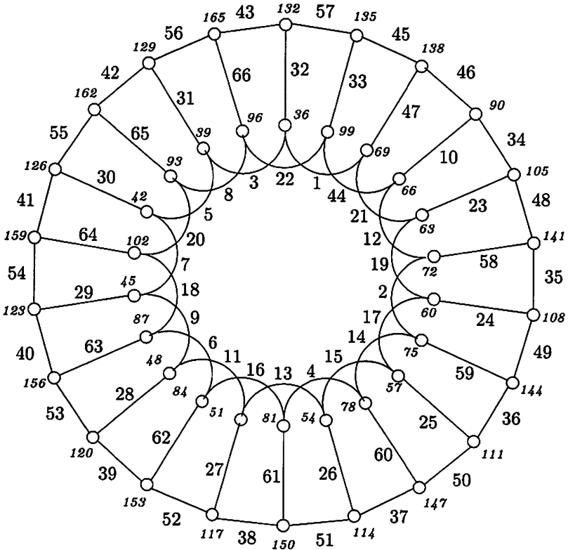
Figure 2.2 : The (\frac{3n+6}{2}, 3) -antimagic labeling of the graph P(22, 2) .
