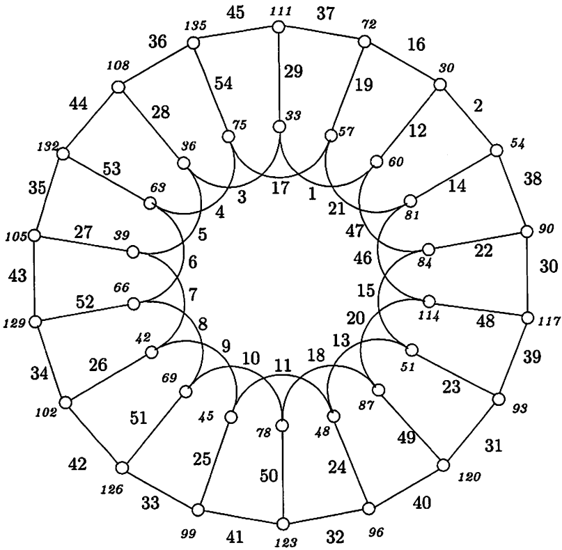
Figure 2.1 : The (\frac{3n+6}{2}, 3) -antimagic labeling of the graph P(18, 2) .
