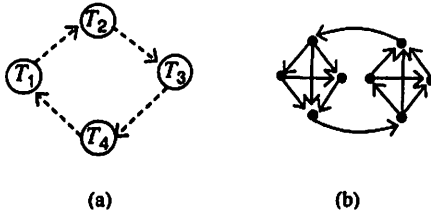
Figure 1: (a) shows an out-tournament where tournaments form one strong component. (b) shows an out-tournament composed of two transitive tournaments.
