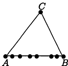
Figure 2. Integral points on the side of a triangle.
