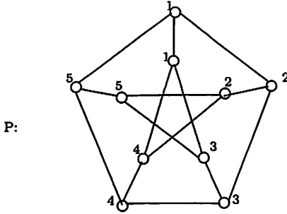
Figure 1: ap(P) = 5
