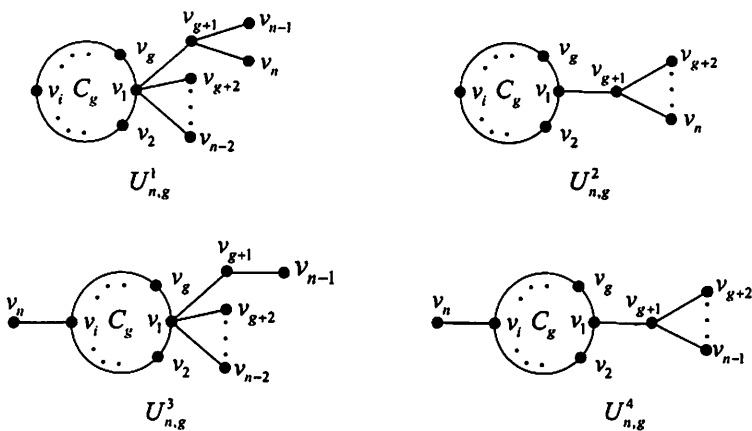
Figure 4: Unicyclic graphs U_{n,g}^1 , U_{n,g}^2 , U_{n,g}^3 and U_{n,g}^4 .
