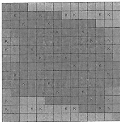
Figure 4: Tiling the Board of Side n = 14
