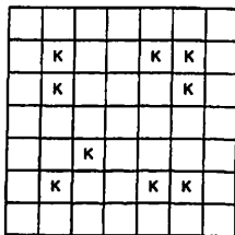
Figure 6: Total Domination on Cube of Side 7
