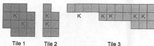
Figure 1: Tiles for Total Domination by Kings
