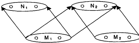
FIGURE 6. A zig-zag of length four.
