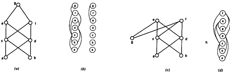
FIGURE 10. The pushdown operation for g lowers the pagenumber from three to two.
