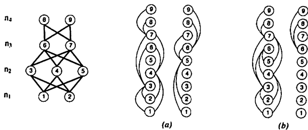
FIGURE 7. A complete multipartite order and a four (a) and three (b) pages book embedding.
