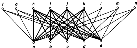
FIGURE 4. A bipartite interval order.
