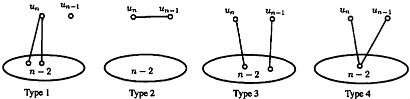
Figure 4: Structure of H in Case 5, Theorem 4.
