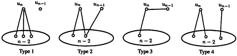
Figure 3: Structure of H in Case 4, Theorem 3.
