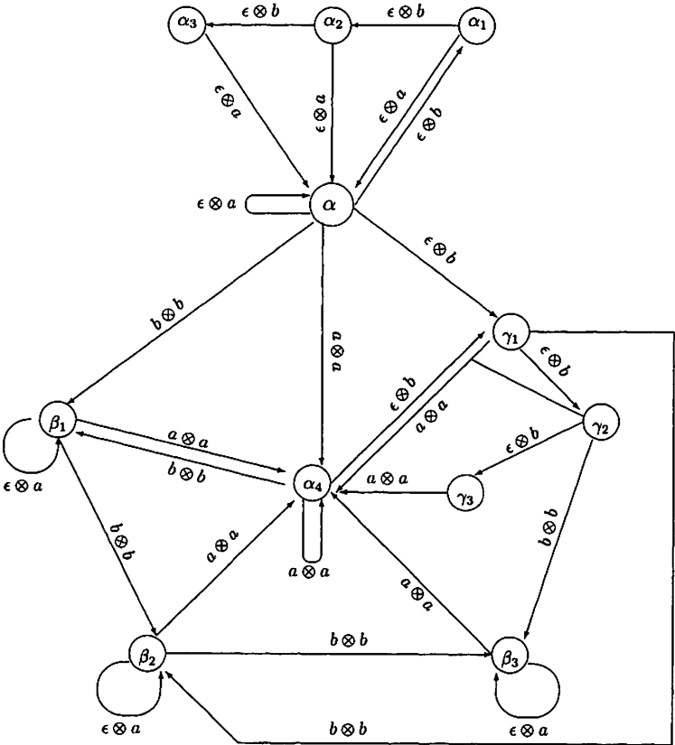
Figure 2: Z_{\otimes}^3
