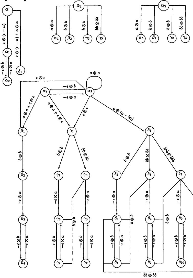
Figure 3: M_{\otimes}^3
