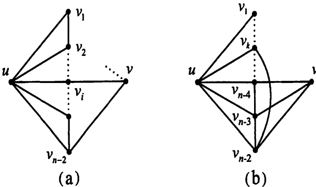
Figure 4: Subgraphs of a Hamiltonian connected graph G with maximum degree n - 2 .
