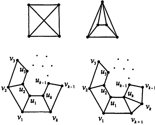
Figure 1: Graph G_n of order n \geq 4 and size \lceil 3n/2 \rceil .
