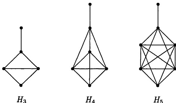
Figure 4: The graphs H_3 , H_4 and H_5 of the family \mathcal{H}
