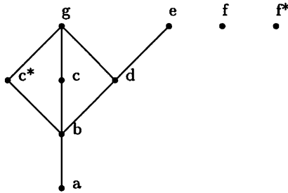
Figure 2: Code inclusions
