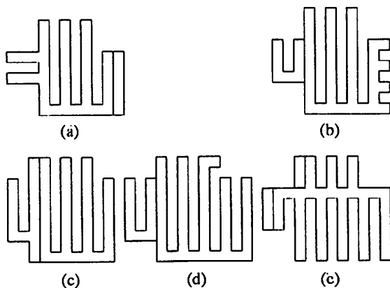
Figure 5: A spanning 2-connected subgraph for : (a) R(10, 12)^{-3(3,3)} with |V| + 1 edges (b) R(11, 12)^{-3(3,3)} with |V| + 1 edges (c) R(11, 13)^{-3(2,2)} with |V| + 1 edges (d) R(11, 13)^{-3(2,3)} with |V| + 1 edges (e) R(11, 13)^{-3(3,3)} with |V| + 2 edges
