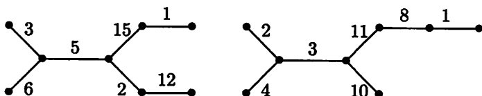
Figure 5: Weighted Trees that Meet M(8)=30
