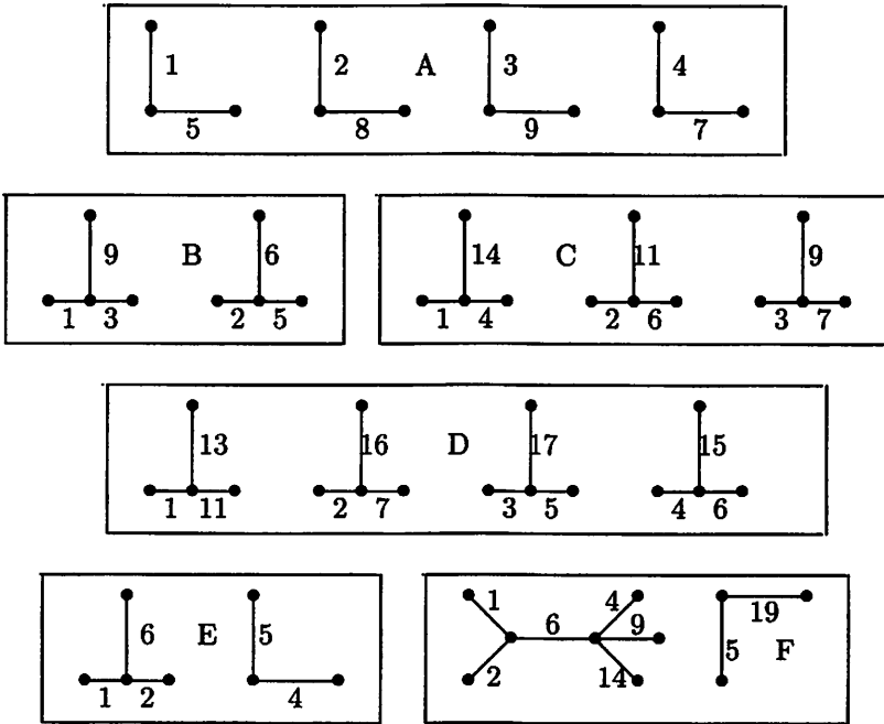
Figure 15: Perfect Distance Forests
