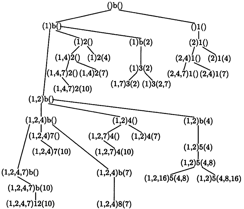
Figure 10: Search Tree for Diameter 3 Trees
