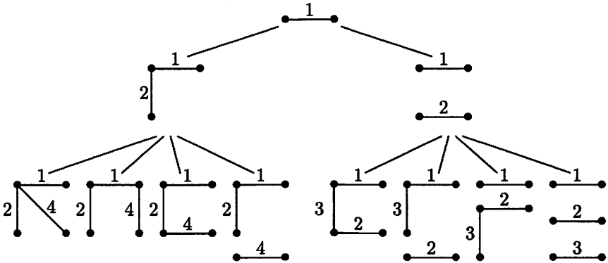
Figure 3: The Search Tree
