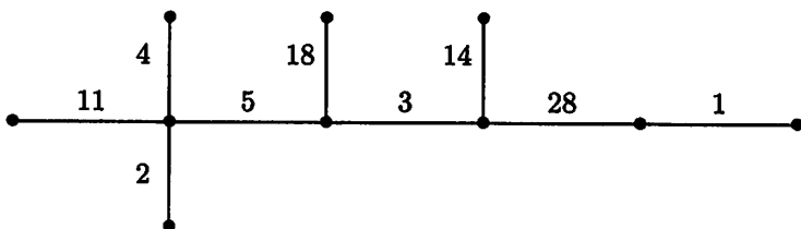
Figure 7: Weighted Trees that Meet M(10)=50
