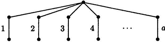
Figure 11: The Diameter 4 Case
