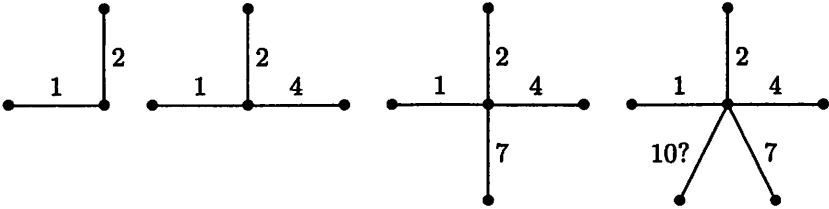
Figure 9: Labeling a Star
