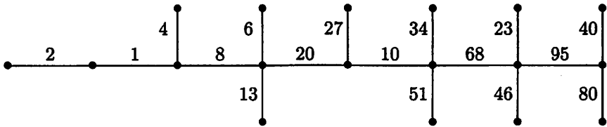
Figure 8: Weighted Tree That Shows M(18) \leq 294
