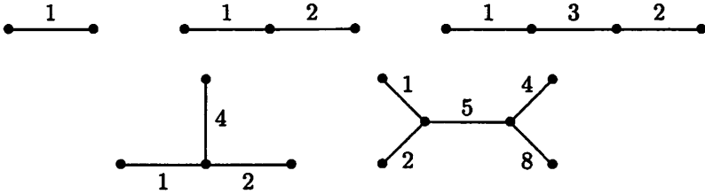
Figure 1: All Known Perfect Distance Trees
