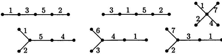
Figure 2: Trees that Meet M(5) = 11
