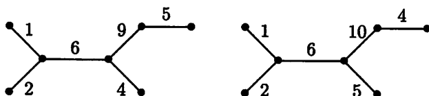
Figure 4: Weighted Trees that Meet M(7)=22
