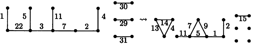
Figure 14: Derivation that is not a Forest
