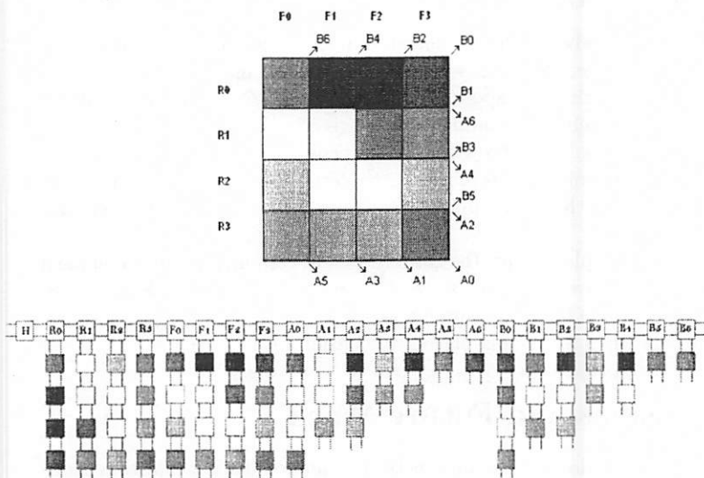
Figure 3: Chessboard and Corresponding Universe
