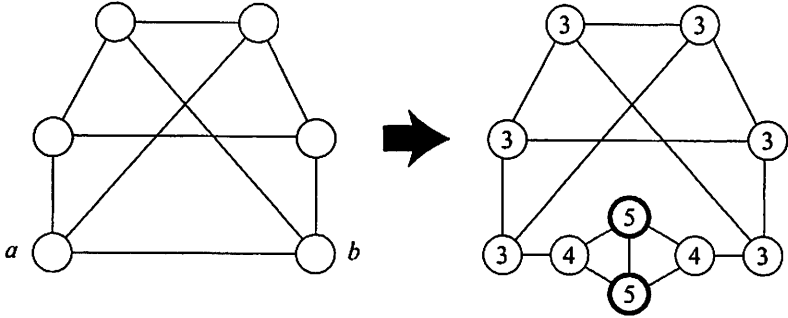
Figure 3: Example for 10 vertices
