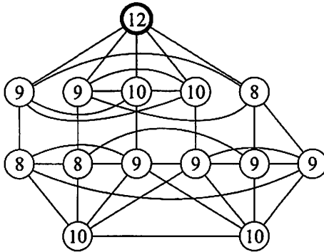
Figure 5: Small quintic graphs, each with a champion
