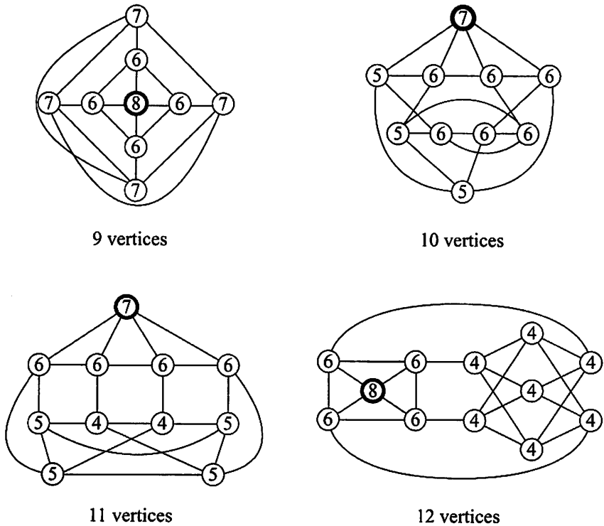
Figure 4: Small quartic graphs, each with a champion
