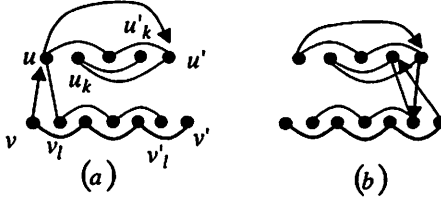
Figure 8: Examples of digraphs and their associated \text{dom}^c(D) graphs where i is odd, j = 2i - 1 , and P_i is a generated subpath on V(P_j) . Edges shown are in \text{dom}^c(D) , while arcs are in D . Bidirected edges are omitted.
