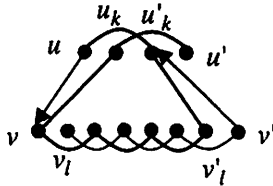
Figure 9: A digraph D where j = 2i on the same set of vertices as \text{dom}^c(D) . Edges shown are those in \text{dom}^c(D) , while arcs are in D . Bioriented edges of D are omitted.
