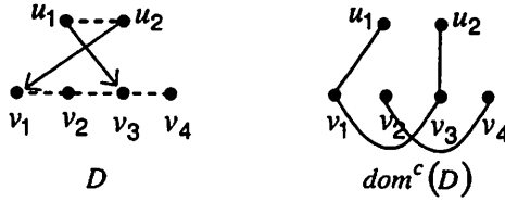
Figure 1: A digraph D where UG^c(D) = P_2 \cup P_4 and the associated graph dom^c(D) . Dashed lines represent UG^c(D) , and bioriented edges of D are omitted.
