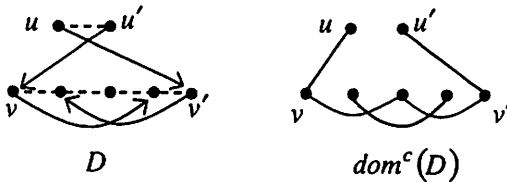
Figure 4: D shows a maximum number of oriented edges when UG^c(D) = P_2 \cup P_5 . Dashed edges are UG^c(D) , and bidirectional edges are omitted for simplicity.
