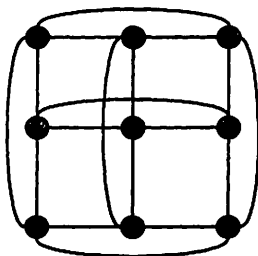
FIGURE 1. The smallest order 2-e.c. graph.
