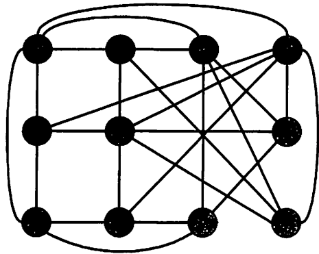
FIGURE 2. The counterexample on 11 vertices.
