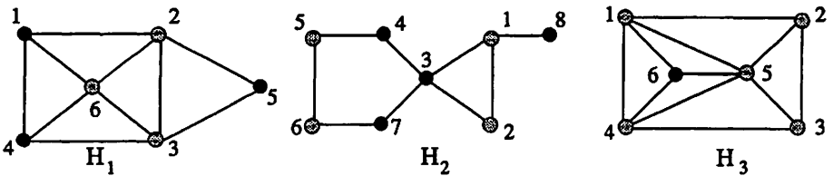
Figure 5: Graphs with (\kappa, \kappa) -regular sets.
