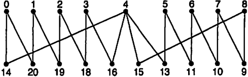
Figure 3: An \alpha -labeling of C_{10} \cup C_{10} .
