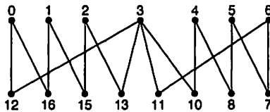
Figure 2: An \alpha -labeling of C_8 \cup C_8 .
