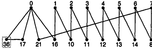
Figure 7: A \gamma -labeling of C_3 \cup C_{16} .
