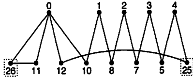
Figure 19: A \rho -tripartite labeling of C_3 \cup C_{11} .
