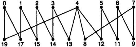
Figure 4: A uniformly-ordered \rho -labeling of C_{10} \cup C_8 .
