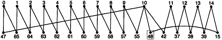
Figure 12: A \gamma -labeling of C_{22} \cup C_{11} .
