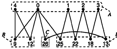
Figure 5: A \gamma -labeling of C_4 \cup C_9 .
