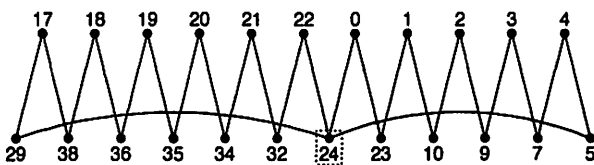
Figure 14: A \sigma -tripartite labeling of C_{13} \cup C_{11} .
