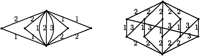
Figure 1: Two balanced directed graphs where the relation on the labeled set \Lambda = \{1, 2, 3\} is the natural linear order. Their respective cd-indexes are 2 \cdot c + 3 and 5 \cdot d . These two examples show that the cd-index of a graph is not necessarily homogeneous and that the coefficient of the c-power term is not necessarily 1.
