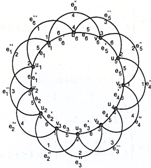
Figure 3: Equitable Total Coloring of total graph of Cycle T(C_6)
