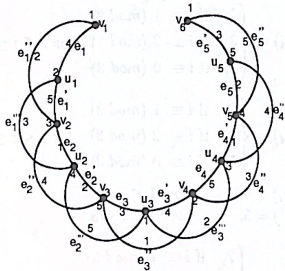
Figure 2: Equitable Total Coloring of total graph of Path T(P_6)
