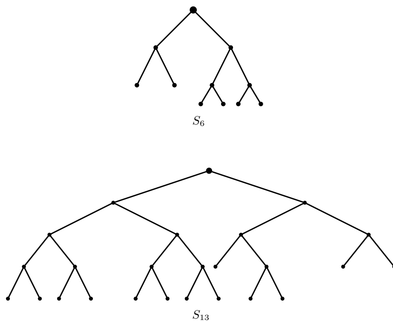
Figure 5: The minimal binary trees S_6 and S_{13} .
