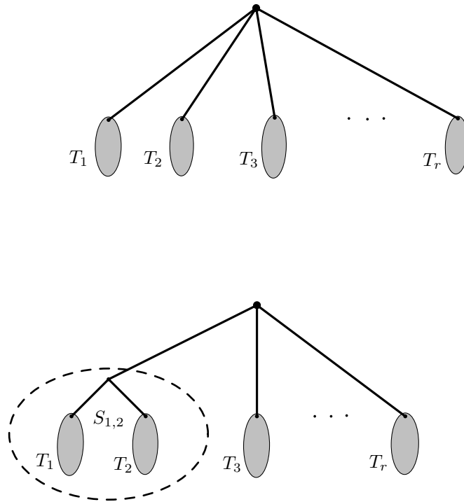
Figure 4: Illustration of the tree transformation F : A topological tree T (top figure) and the corresponding tree F(T) (bottom figure).
