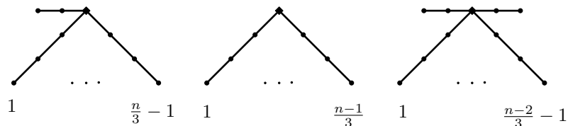
Figure 2: The minimal trees among all n -vertex rooted trees according to the residue of n modulo 3 (the root is the square vertex on top) [9].
