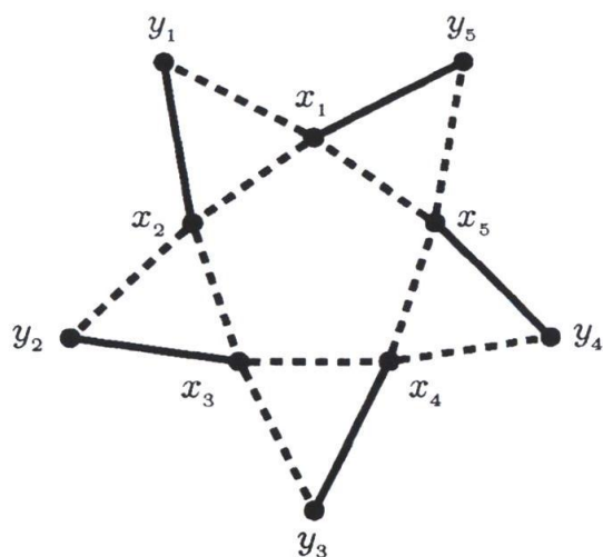
Figure 8: A signed K_4 -minor-free graph which does not map to \text{EDC}(SPal_5)
