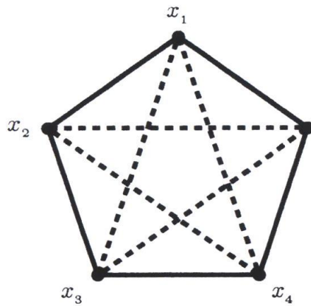
Figure 1: SPal_5
