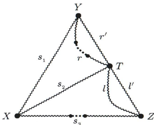
Figure 6: Bipartite subdivision of a negative even cycle with 3 chords
