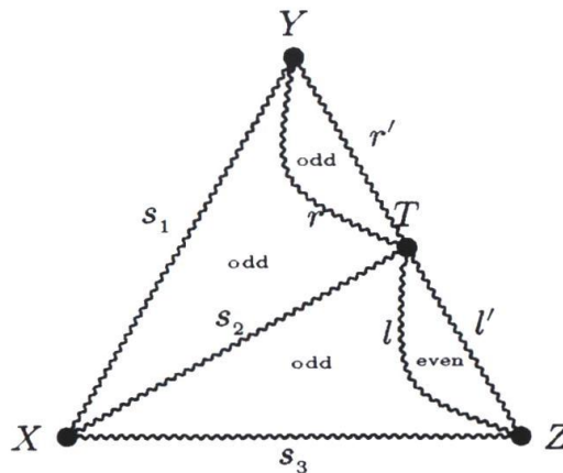
Figure 5: Subdivision of a C_{2k+1} -cycle with 3 chords
