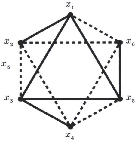
Figure 2: A 6-vertices bound for the class SSPG
