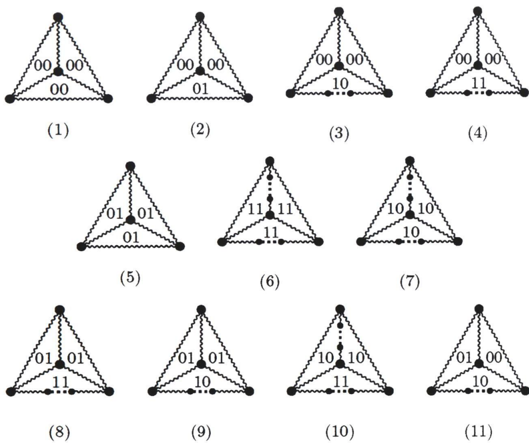
Figure 3: Classification of signed K_4 -subdivisions
