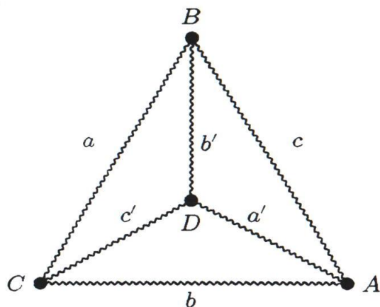
Figure 4: Labeling a K_4 -subdivision
