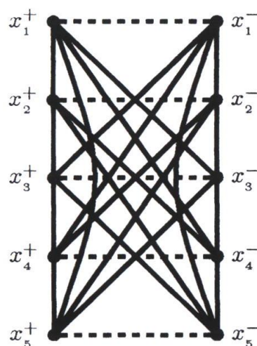
Figure 7: \text{EDC}(SPal_5)
