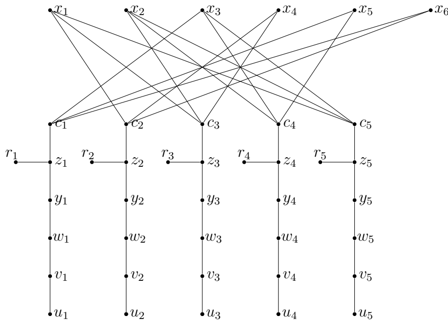
Fig. 1. NP-completeness of vertex-edge locating Roman domination for bipartite graphs
