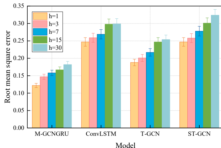
Fig. 5. Prediction accuracy of the optimal model at each step size
