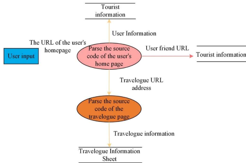
Fig. 1. Single user crawling data flow
