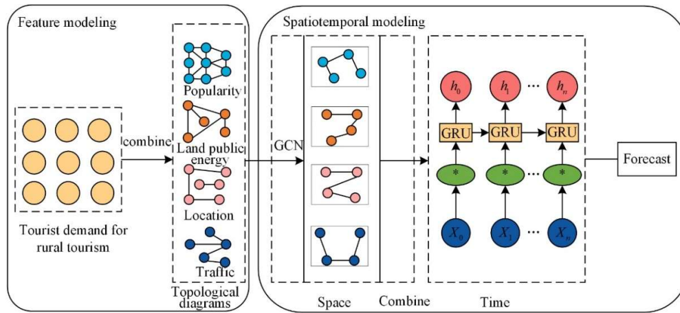
Fig. 3. Tourist behavior analysis and prediction framework for rural tourism scenic spots
