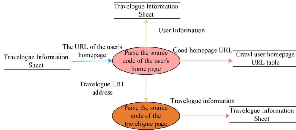
Fig. 2. Database batch crawling module
