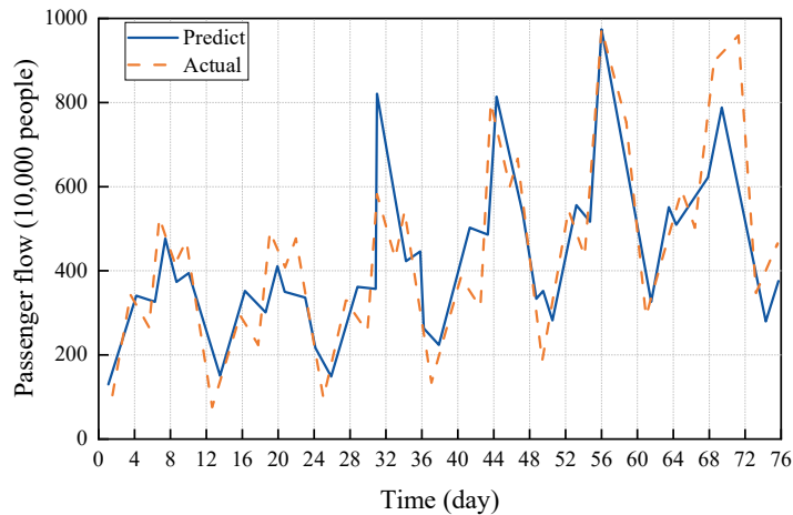
Fig. 6. Forecast results of tourist volume of rural attractions
