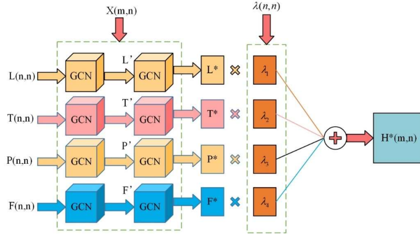
Fig. 4. Spatial dependence model
