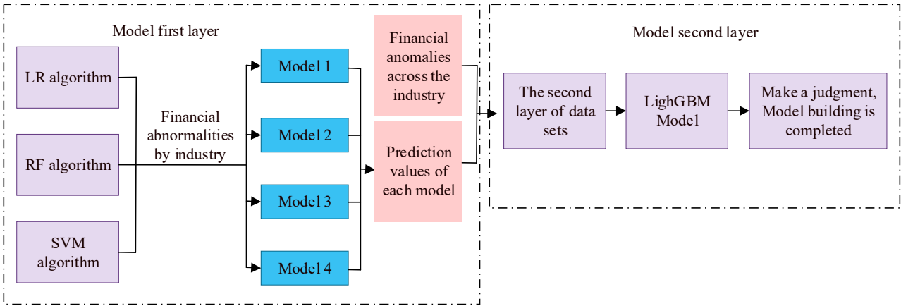
Fig. 3. Intelligent financial statement anomaly recognition based on multi-source data
