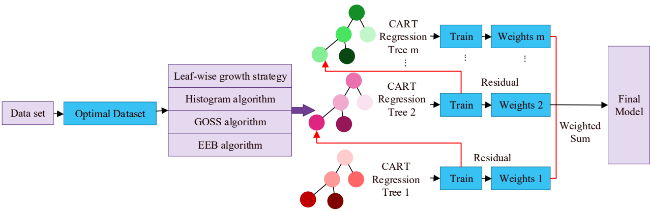
Fig. 2. LightGBM algorithm flow
