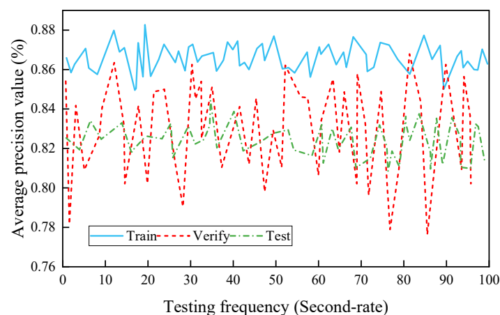
Fig. 4. Average precision value of fusion multi-source data sets
