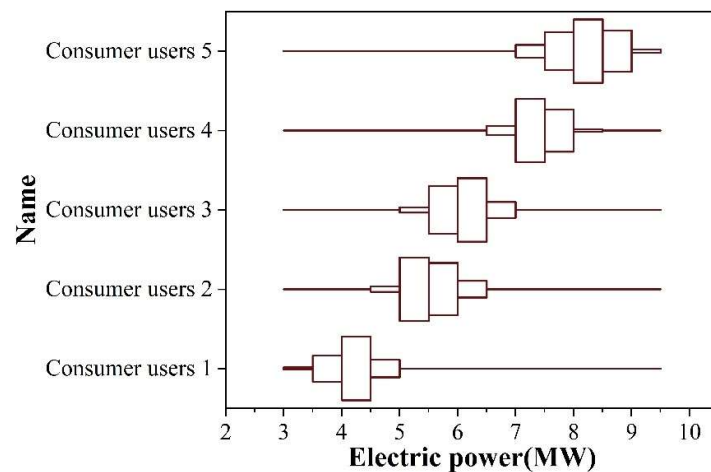
Fig. 9. Consumer users consume gas power
