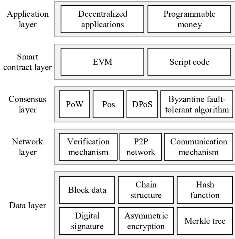
Fig. 1. Heterogeneous blockchain
