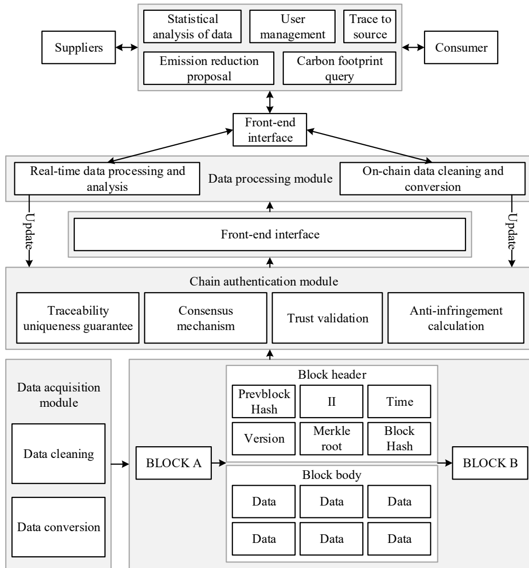
Fig. 3. Carbon footprint retracing mechanism design
