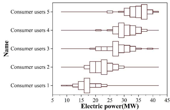
Fig. 8. Consumer users consume thermal power
