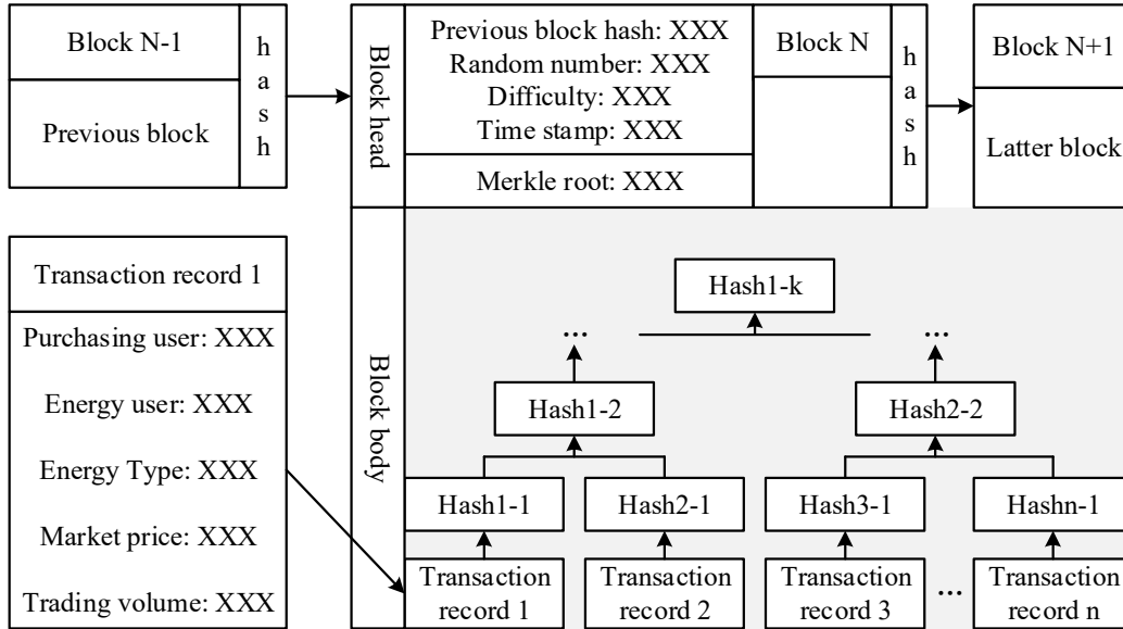
Fig. 2. Block data structure
