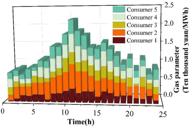
Fig. 14. Thermal energy utility parameters of \alpha_i^{GP} consumptive users
