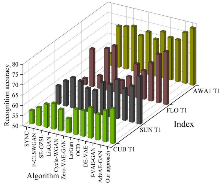
Fig. 3. The accuracy of the zero sample image recognition in four data sets
