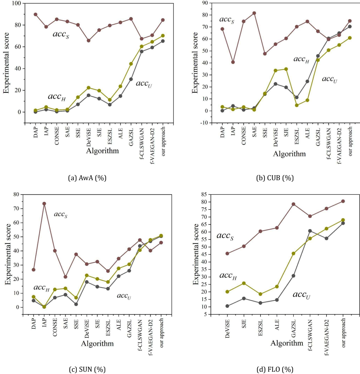
Fig. 4. The results of the generalized zero-sample study in this paper
