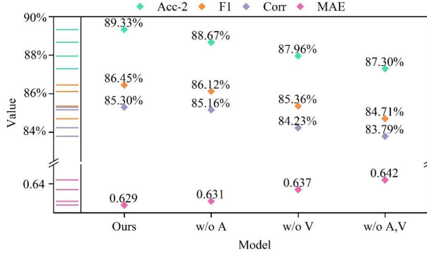
Fig. 7. Ablation Study of this model
