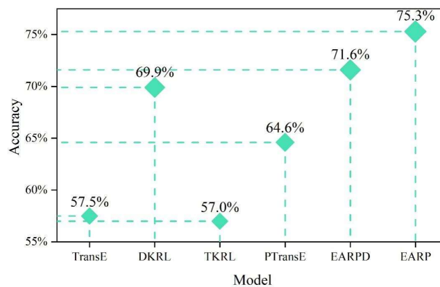
Fig. 8. Results of the triples experiment
