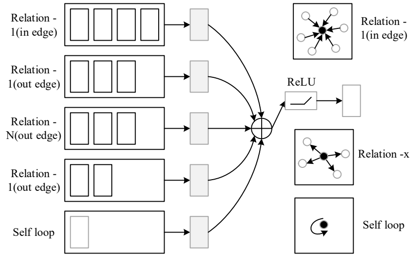
Fig. 3. Node update process in multi-graph encoder
