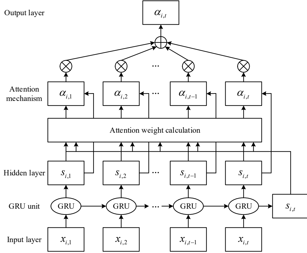
Fig. 5. Structure of timing encoder
