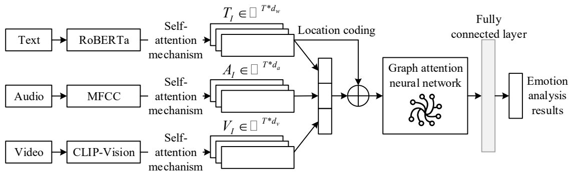
Fig. 2. Multi-modal emotion analysis based on graph attention neural network
