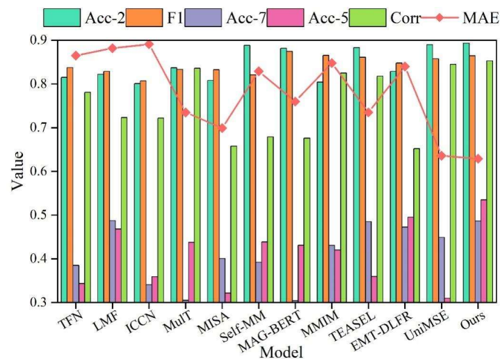
Fig. 6. Experimental Results of this model on CMU-MOSI
