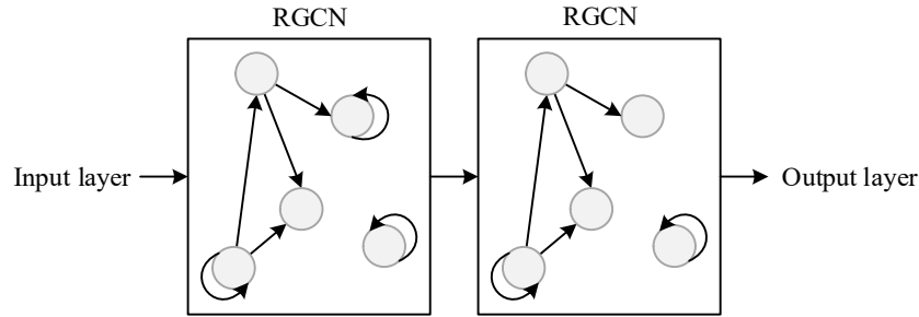
Fig. 4. Schematic diagram of convolutional neural network(RGCN)encoder
