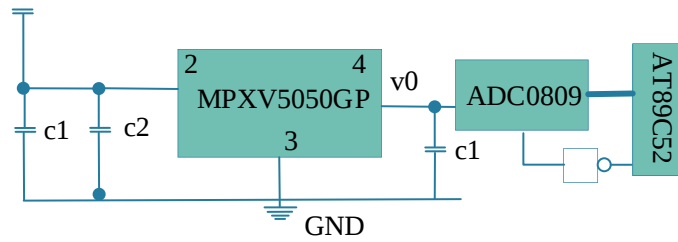
Fig. 2. MPXV5050GP and its peripheral circuits
