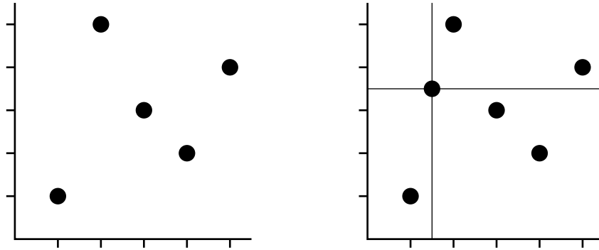
Figure 2: ins(15324, 2, 4) = 146325 .
